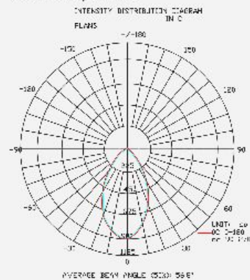
Photometry 4000K
