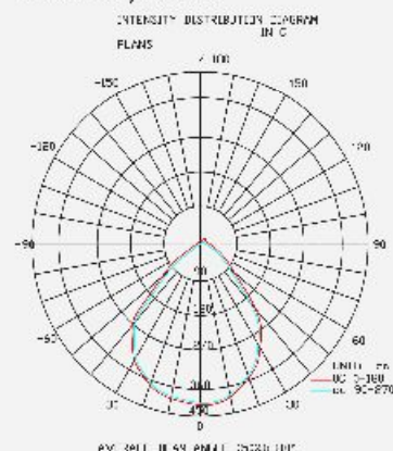
Photometry 4000K
