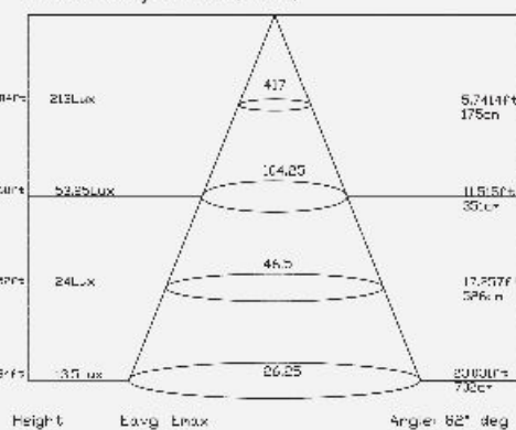
Photometry 4000K ( 100° )
