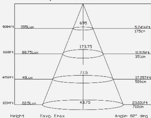
Photometry 4000K ( 100° )
