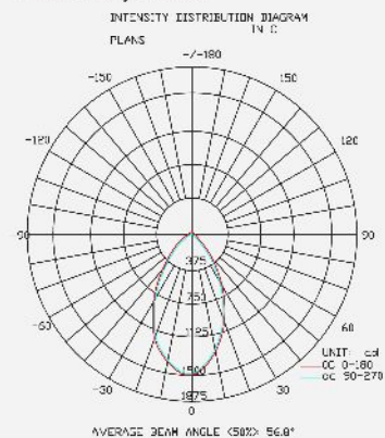
Photometry 4000K
