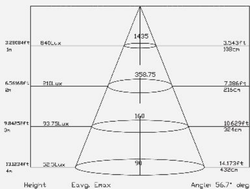
Photometry 4000K ( 66° )
