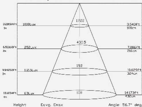
Photometry 4000K ( 66° )
