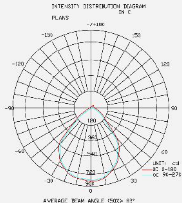
Photometry 4000K
